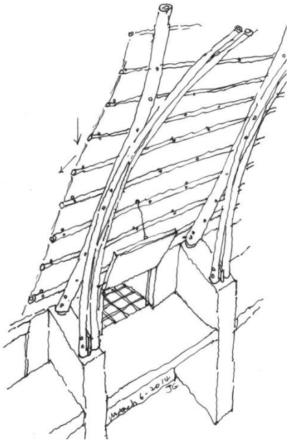
Kitchen interior door to cooking caustic zone in the exterior reflector box
